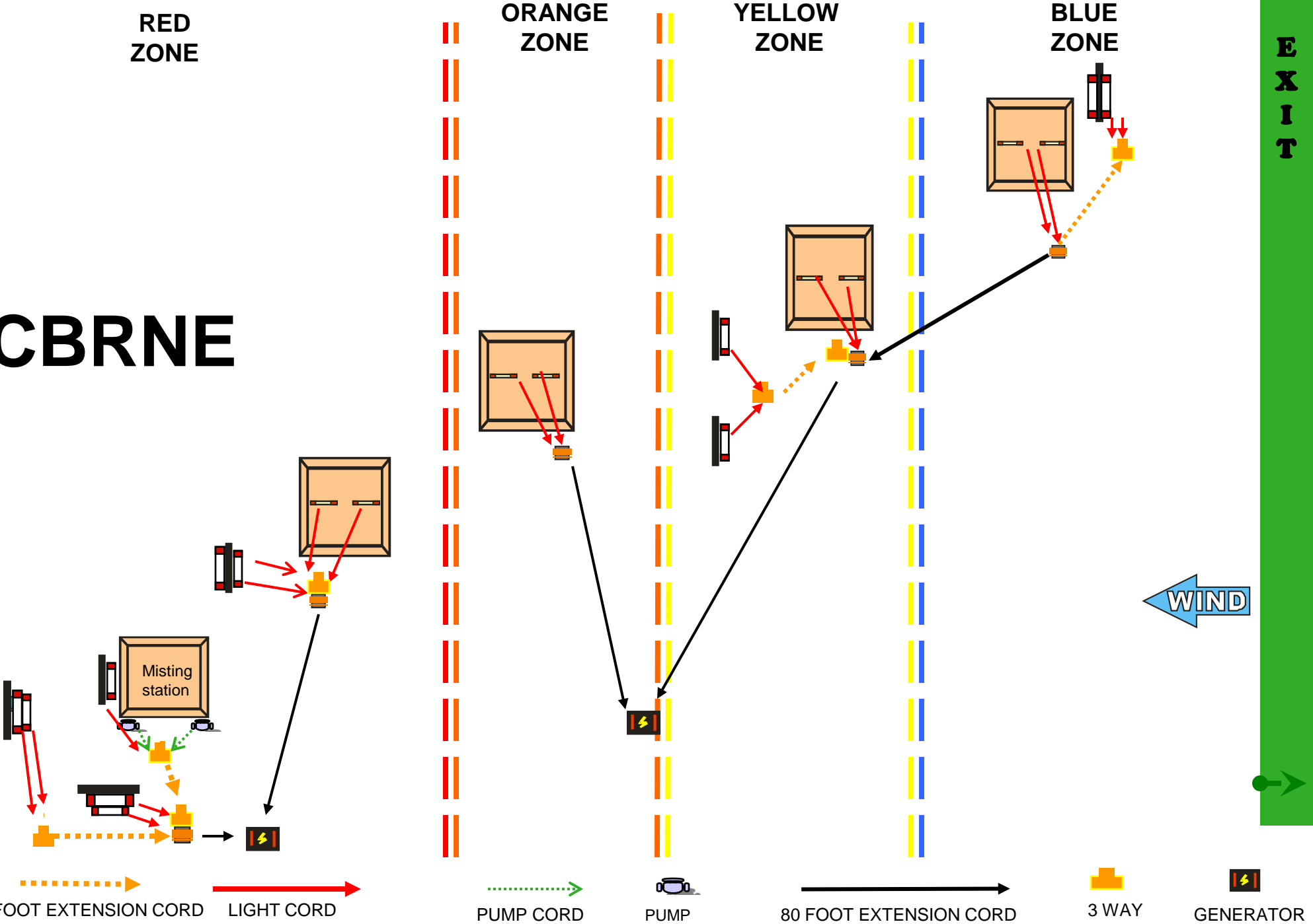
Electrical setup
